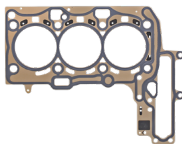
597.120 # 11 12 8 511 228 1,10 mm | 3-layer
