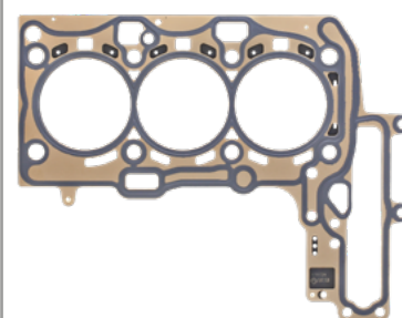
597.130 # 11 12 8 511 229 1,20 mm | 3-layer
