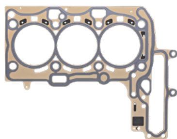
597.110 # 11 12 8 511 227 1,00 mm | 3-layer
