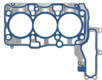
192.660 # 11 12 8 594 564 1,55 mm | 3-layer
