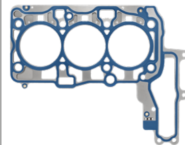
192.670 # 11 12 8 594 565 1,65 mm | 3-layer
